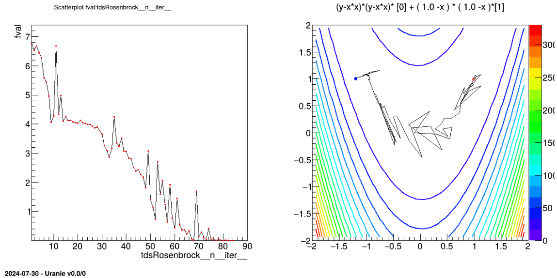
Figure XIV.77: Graph of the macro "optimizeCodeRosenbrockKeyRowRecreate.C"
