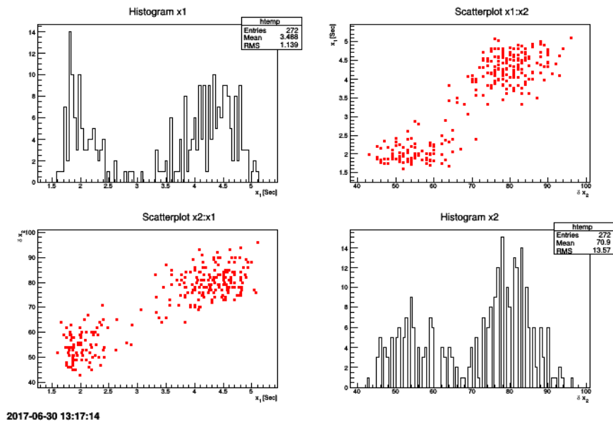
Figure II.49: Graphs of "Tuft" type between the attributes x1 and x2 of the TDataServer geysers.
