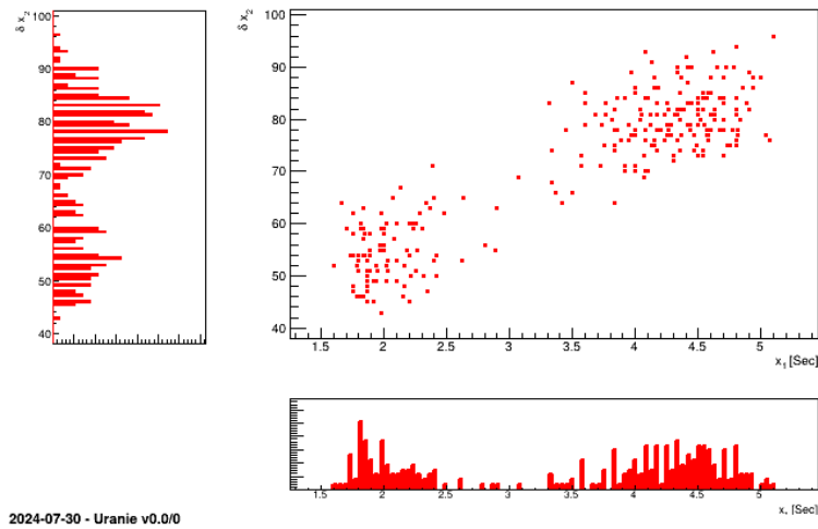
Figure II.48: Graphs of "Tuft" type between the attributes x1 and x2 of the TDataServer geysers.
