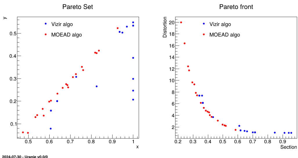
Figure XIV.93: Graph of the macro "reoptimizeHollowBarVizirMoead.C"
