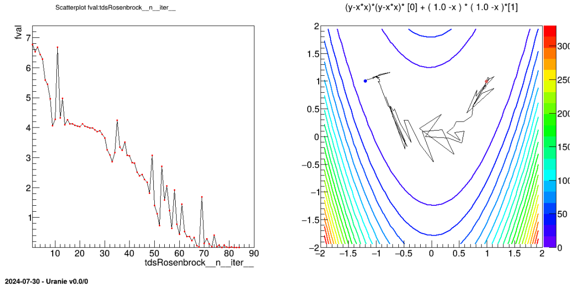
Figure XIV.74: Graph of the macro "optimizeCodeRosenbrockKey.C"
