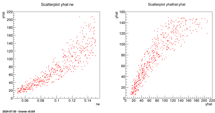
Figure XIV.64: Graph of the macro "modelerFlowrateLinearRegression.C"
