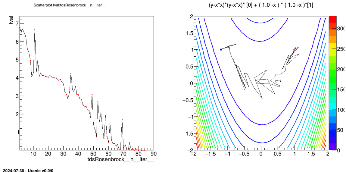
Figure XIV.76: Graph of the macro "optimizeCodeRosenbrockRow.C"
