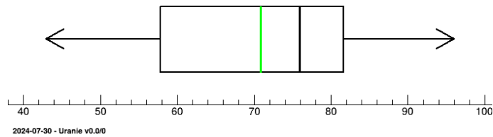
Figure II.43: Boxplot of attribute x2 of the TDataServer geyser
