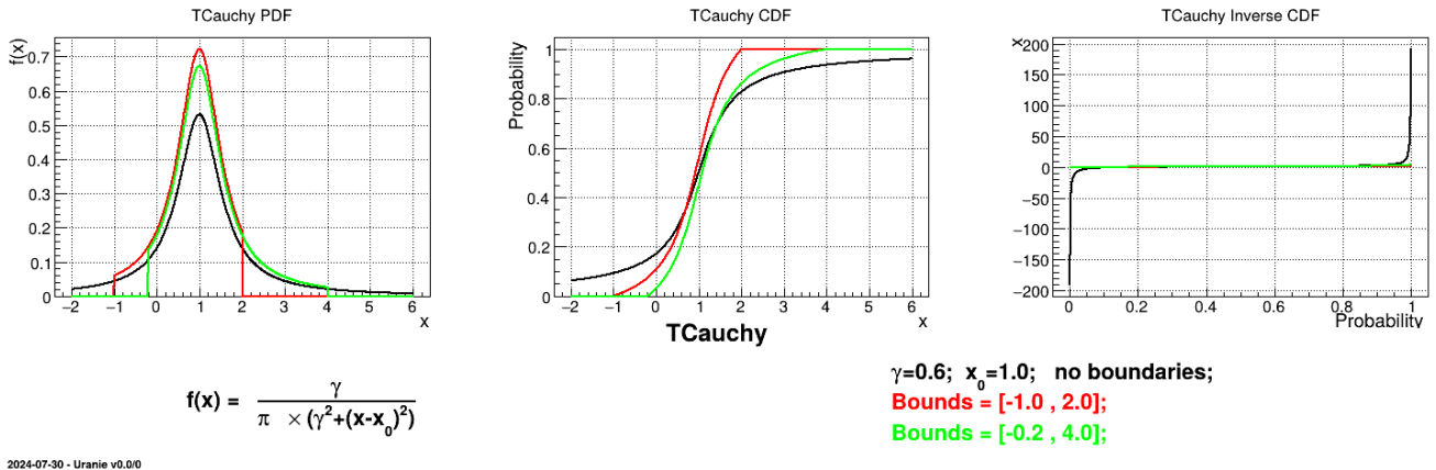
Figure II.18: Example of PDF, CDF and inverse CDF for a Cauchy truncated distribution.
