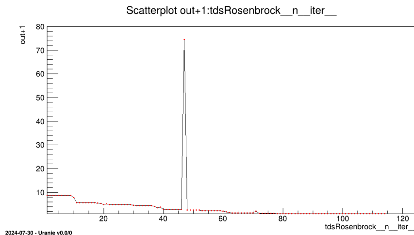
Figure XIV.73: Graph of the macro "optimizeFunctionRosenbrockNewInputOutput.C"
