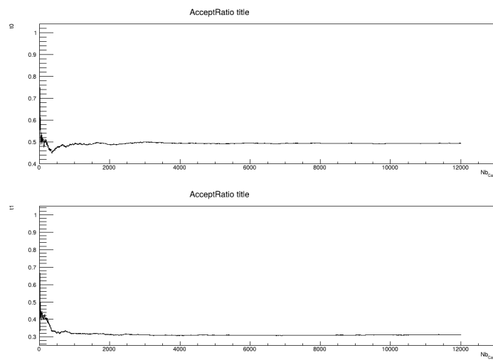
Figure XIV.105: Acceptation rate graph of the macro "calibrationMetropHastingLinReg.C"
