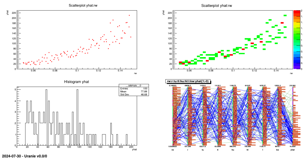
Figure XIV.29: Graph of the macro "launchCodeFlowrateKeywithFlagSampling.C"
