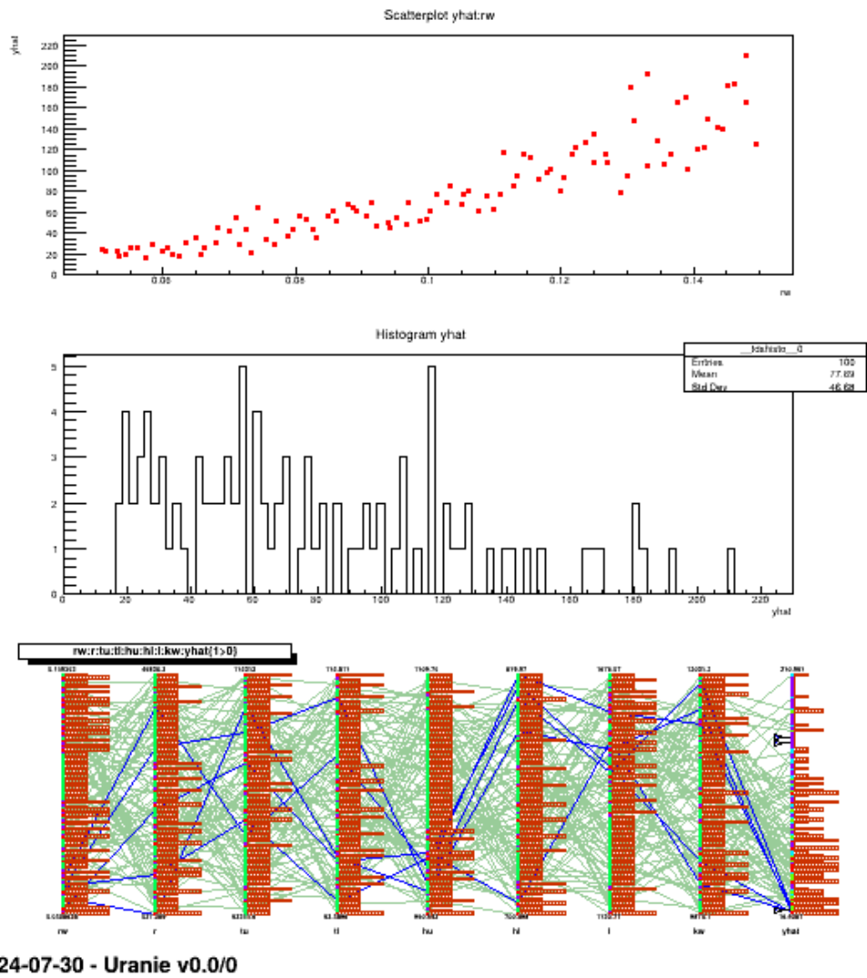
Figure XIV.25: Graph of the macro "launchCodeFlowrateKeyRecreateSamplingOutputDataServer.C"
