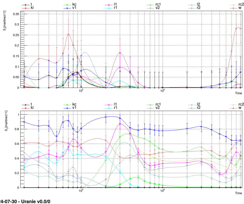
Figure XIV.54: Graph of the macro "sensitivitySobolLeveLE.C"
