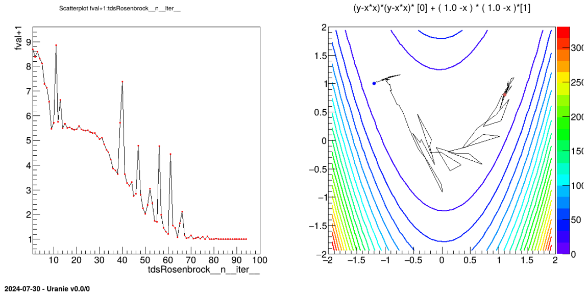
Figure XIV.75: Graph of the macro "optimizeCodeRosenbrockKeyNewInputOutput.C"
