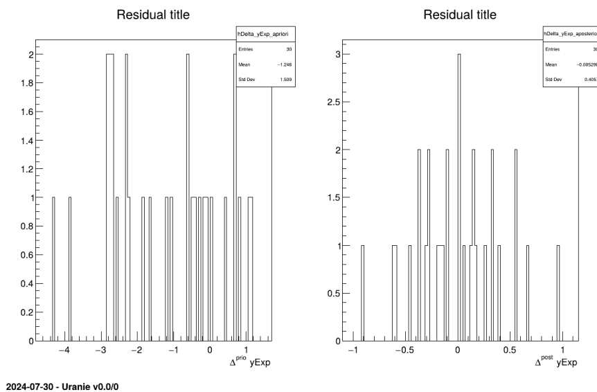
Figure XIV.106: Residual graph of the macro "calibrationMetropHastingLinReg.C"
