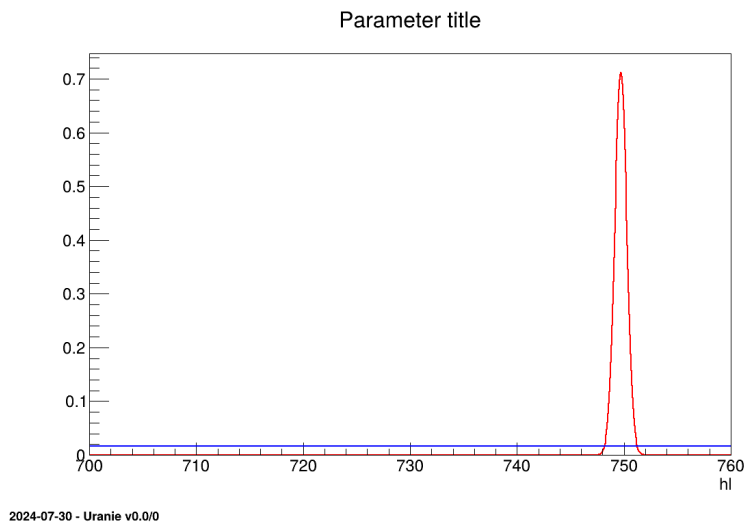
Figure XIV.98: Parameter graph of the macro "calibrationLinBayesFlowrate1D.C"
