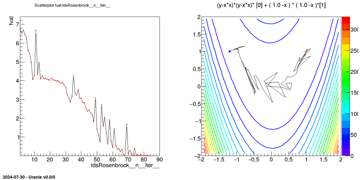
Figure XIV.79: Graph of the macro "optimizeCodeRosenbrockRowRecreateOutputDataServer.C"
