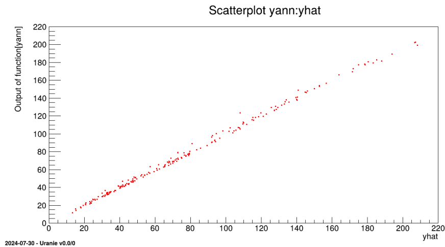
Figure XIV.66: Graph of the macro "modelerFlowrateNeuralNetworks.C"
