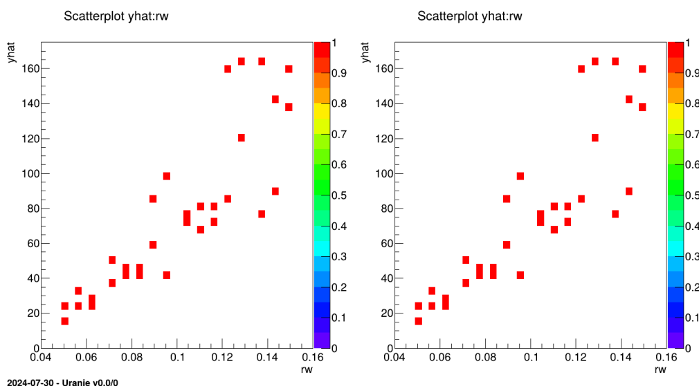
Figure XIV.87: Representation of the output as a function of the first input with a colZ option when using either the classical or dedicated constructor
