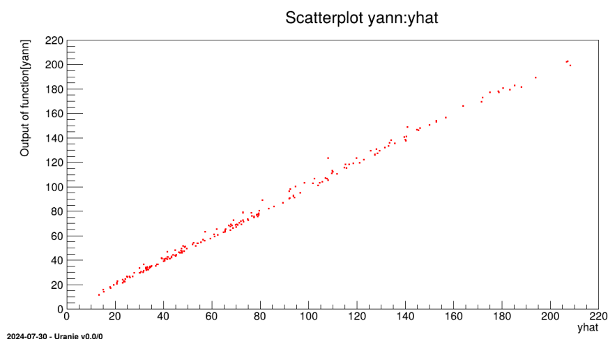
Figure XIV.67: Graph of the macro "modelerFlowrateNeuralNetworksLoadingPMML.C"
