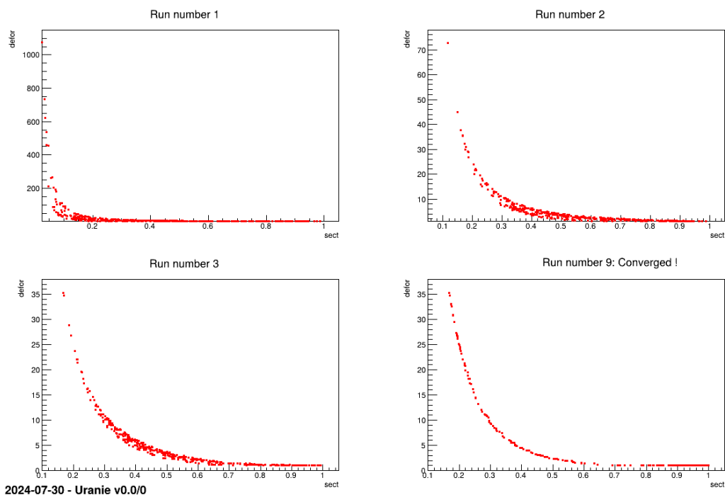
Figure XIV.94: Graph of the macro "reoptimizeHollowBarVizirSplitRuns.C"
