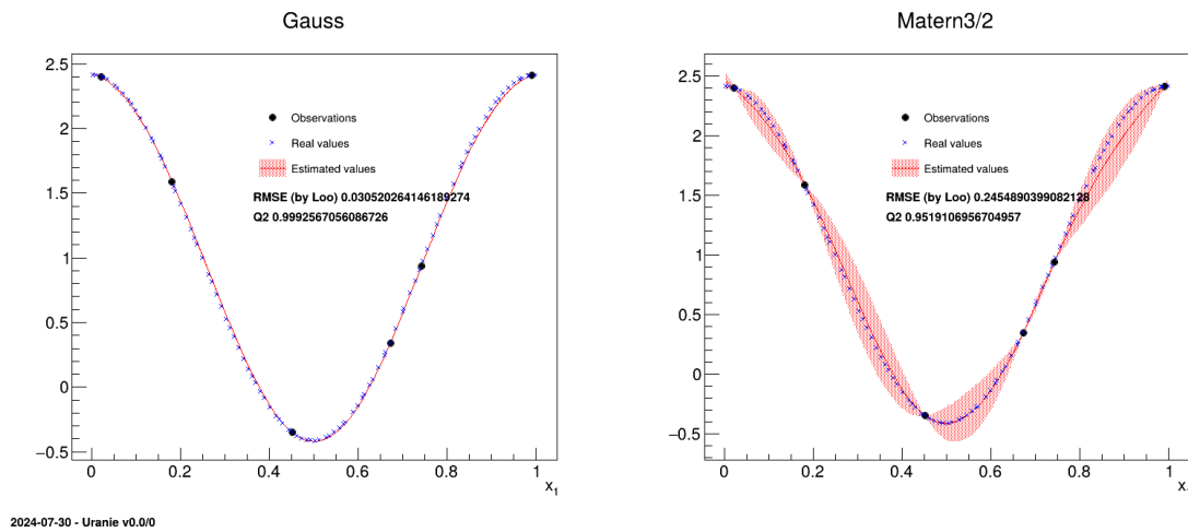
Figure XIV.71: Graph of the macro "modelerTestKriging.C"
