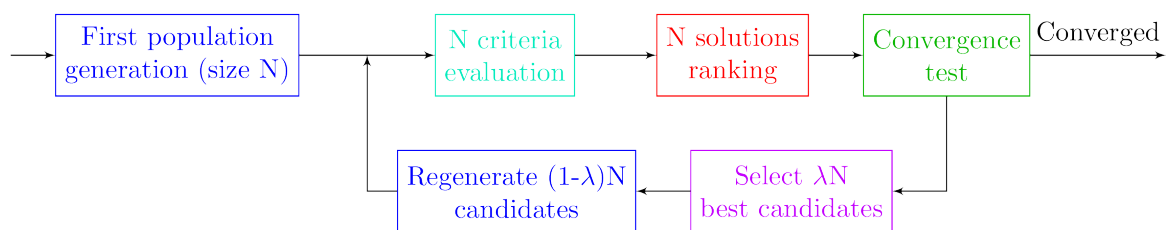
Figure IX.2: Schematic description of the requested steps of an optimisation procedure once this one is performed with Vizir
