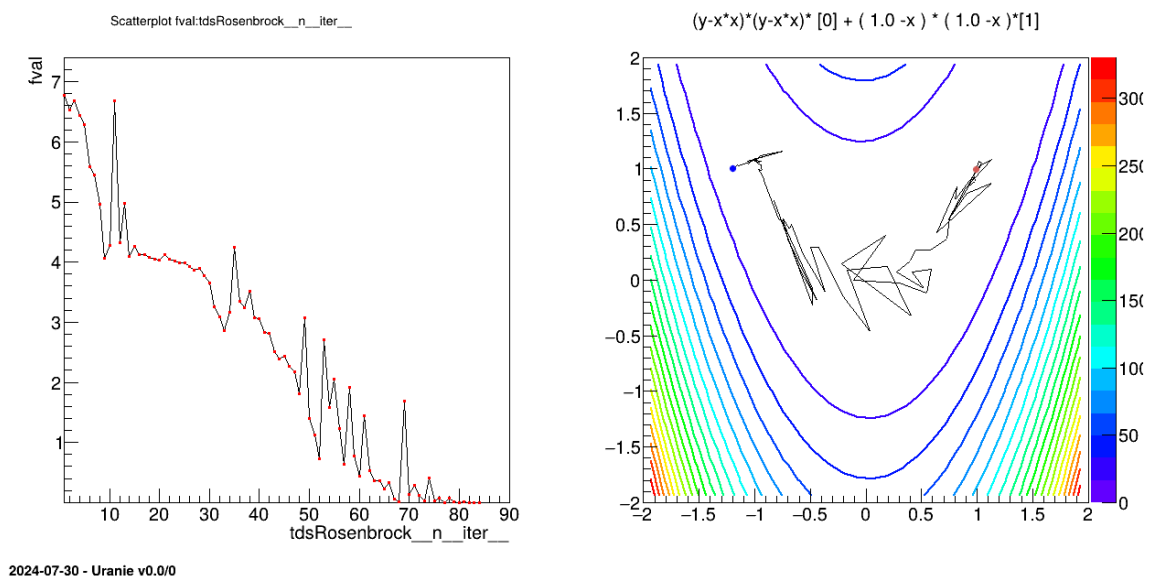
Figure XIV.78: Graph of the macro "optimizeCodeRosenbrockRowRecreate.C"
