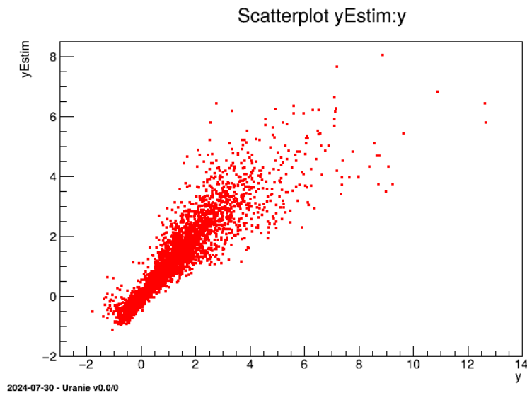
Figure XIV.69: Graph of the macro "modelerbuildSimpleGPEstim.C"
