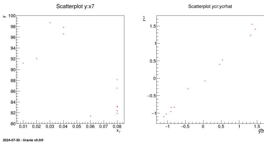
Figure XIV.63: Graph of the macro "modelerCornellLinearRegression.C"
