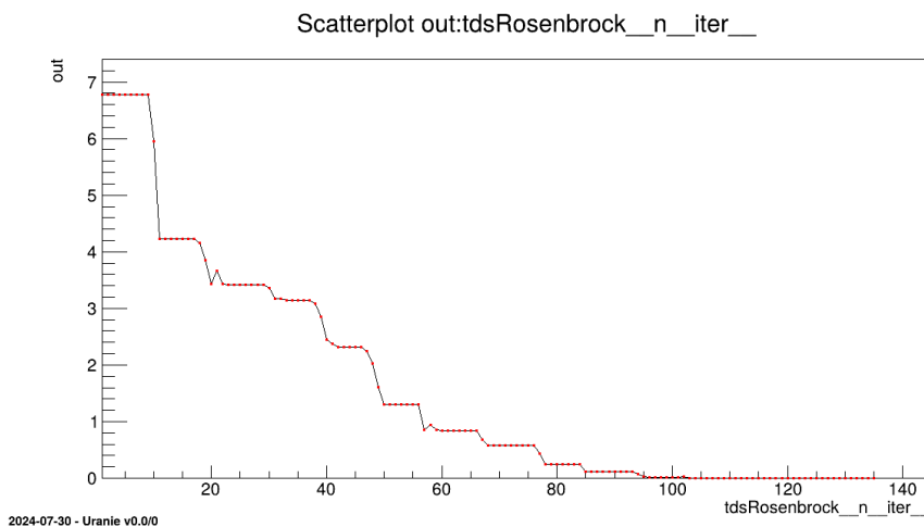
Figure XIV.72: Graph of the macro "optimizeFunctionRosenbrock.C"
